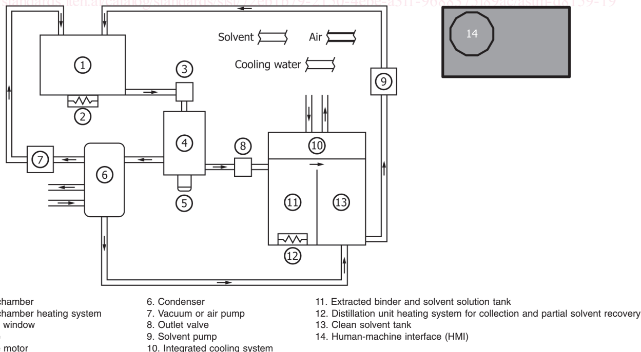
FIG. 1 Schematic Drawing of Automated Extraction Unit
