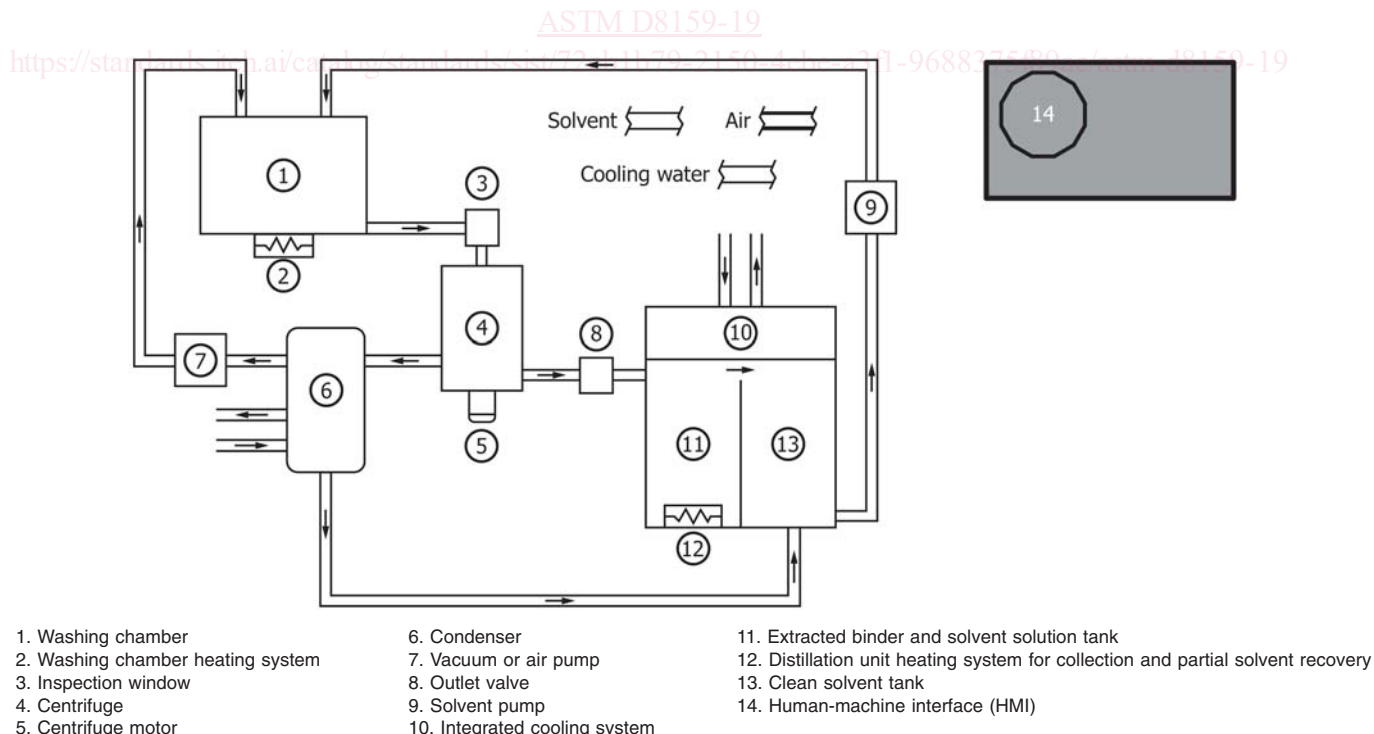
FIG. 1 Schematic Drawing of Automated Extraction Unit
