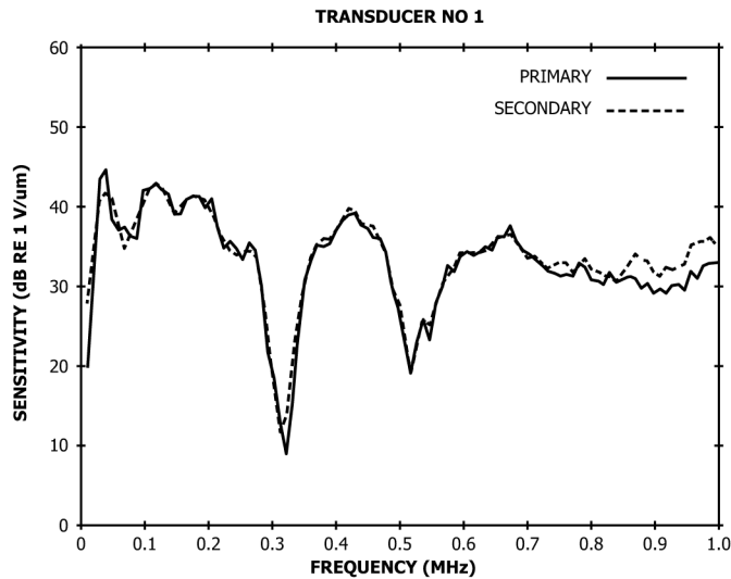
FIG. 2 Comparison of Primary and Secondary Calibration Results for a SUT Having a Nominal Diameter of 12.7 mm (0.5 in.)
