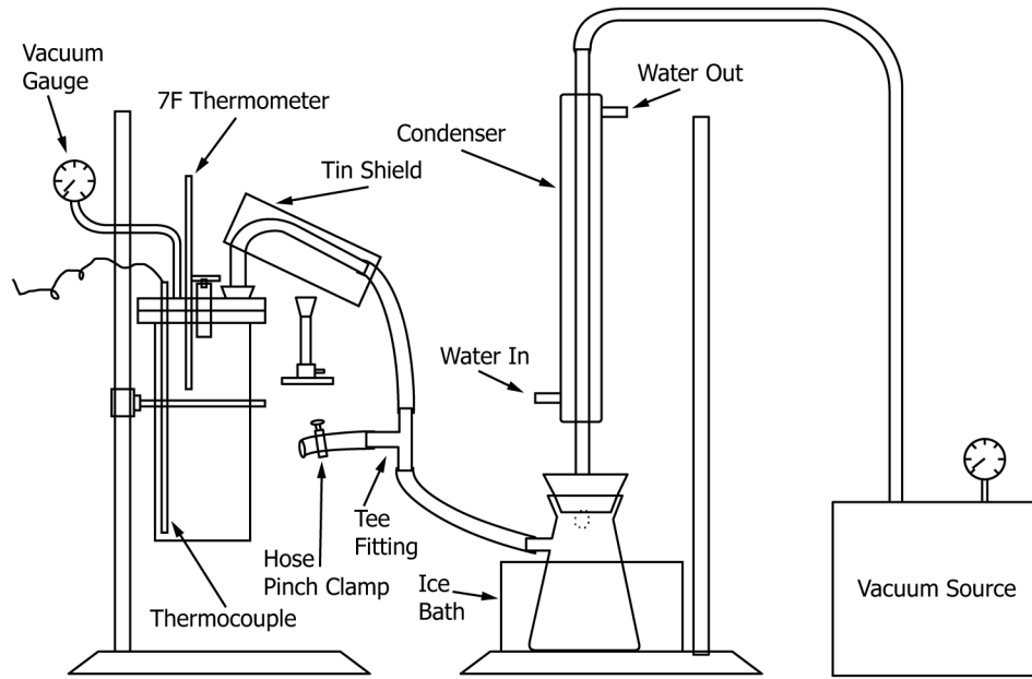
FIG. 2 Connection Apparatus Schematic
