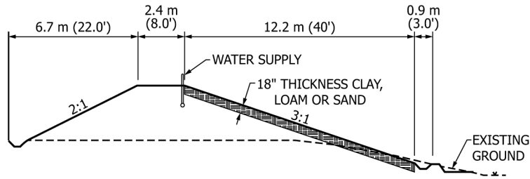
FIG. 2 Typical Embankment Cross Section
