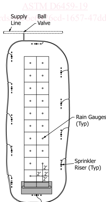
FIG. 4 Typical Sprinkler Riser Configuration
