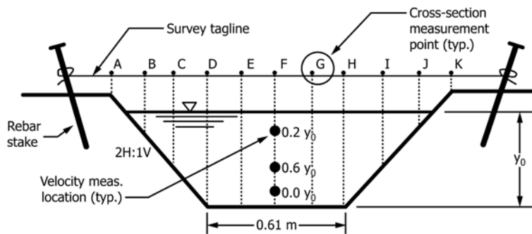
FIG. 3 Typical Channel Cross Section
