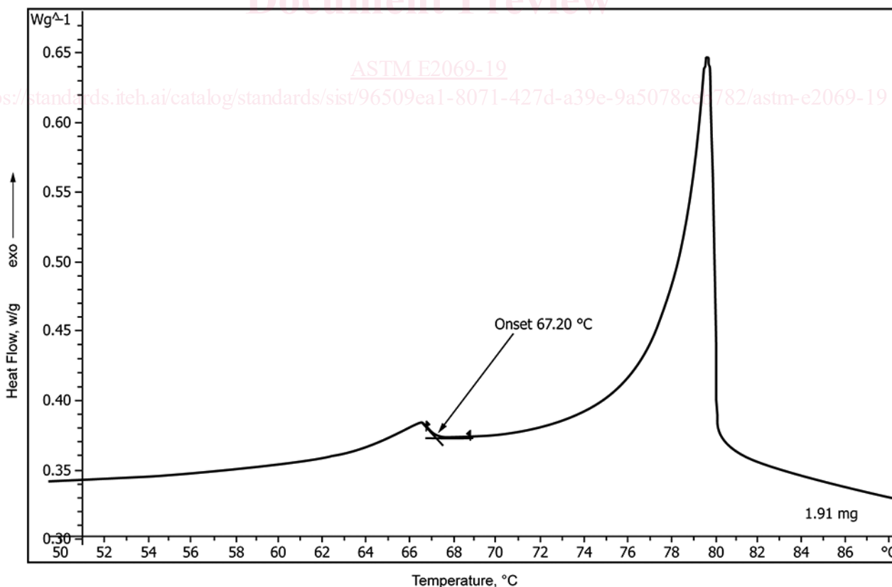
FIG. 1 Cooling Curve for M-24
