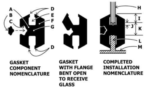
FIG. 4 Gasket Mounting Clearance
