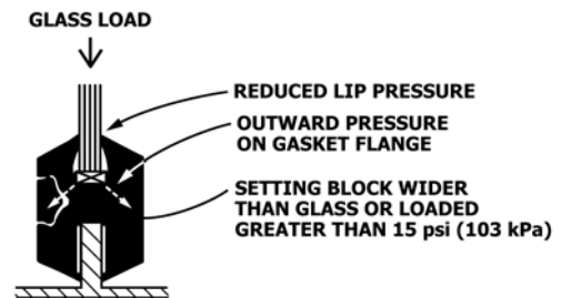
FIG. 10 Effect on Gasket Caused by Too Wide or Overloaded Setting Blocks
