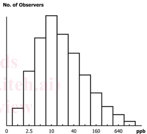
FIG. 3 Skewed Distribution
