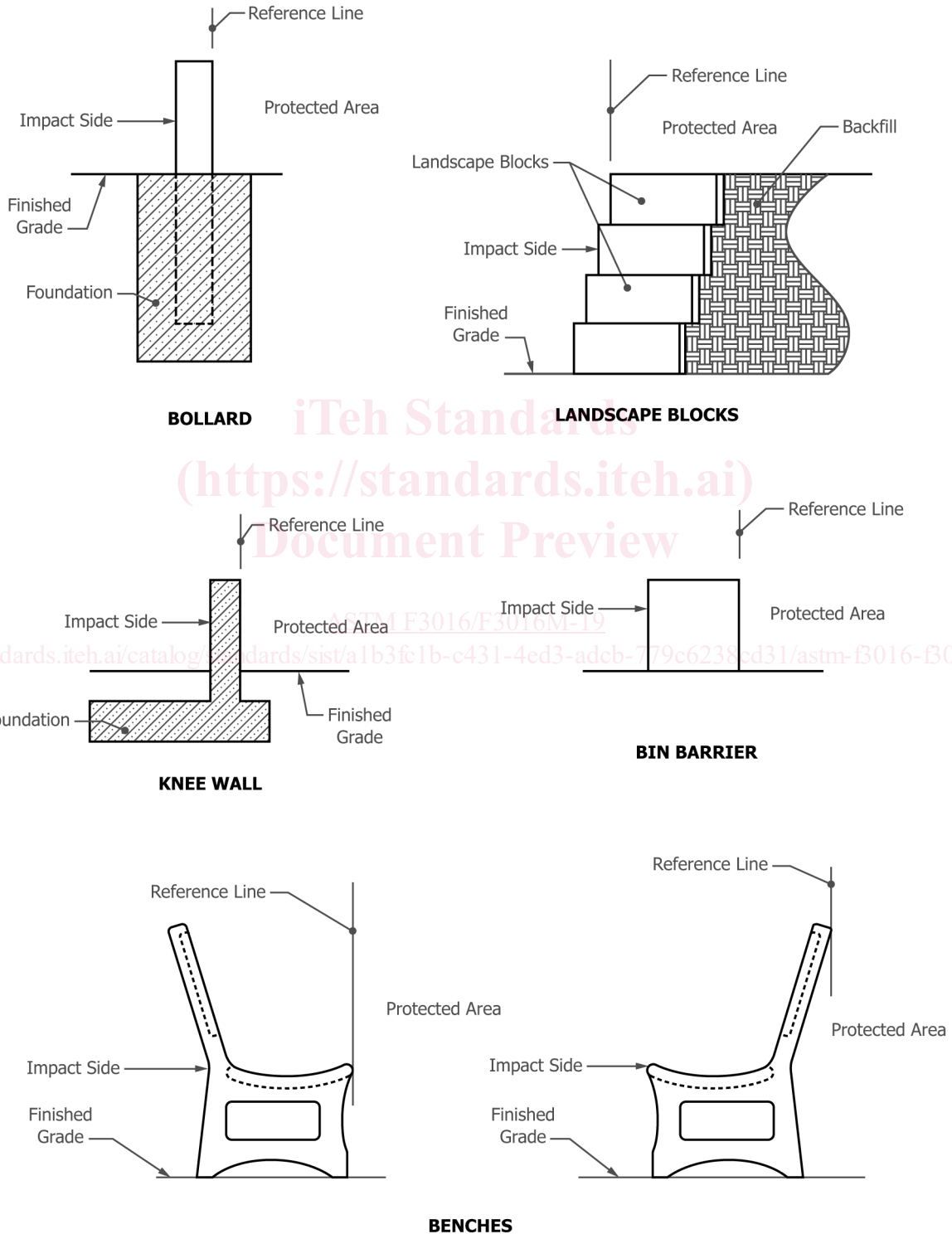
FIG. A1.1 Protective Devices Reference Locations
