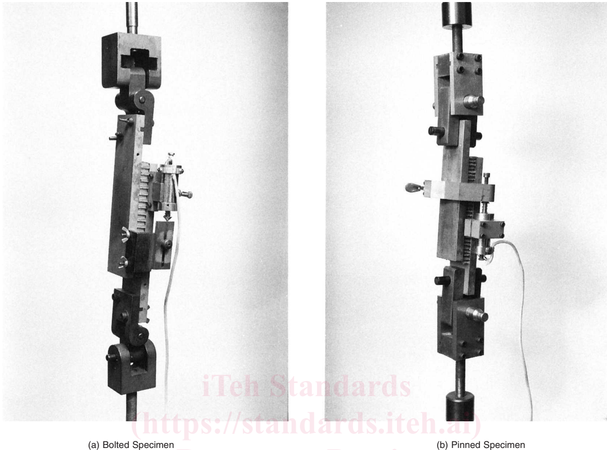
FIG. 23 Tensile Plate Shear Test Set Up
