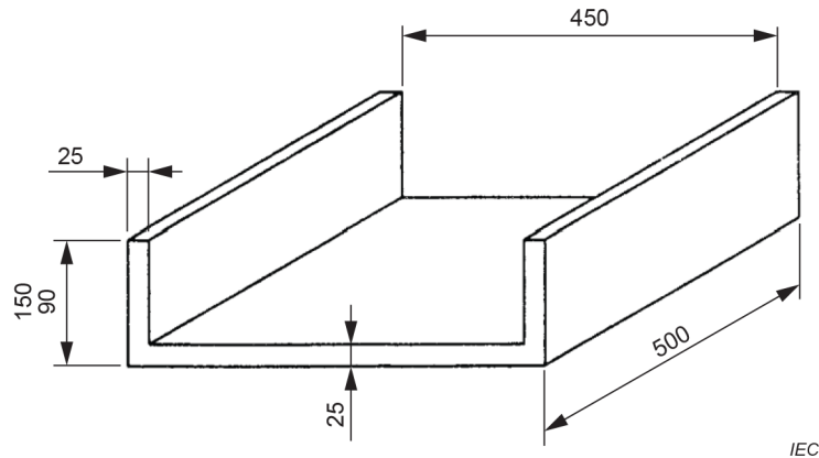
Figure 2 – Yoke dimensions
