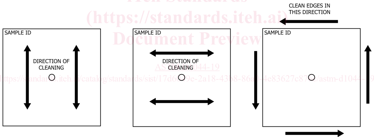
FIG. 4 Specimen Cleaning
