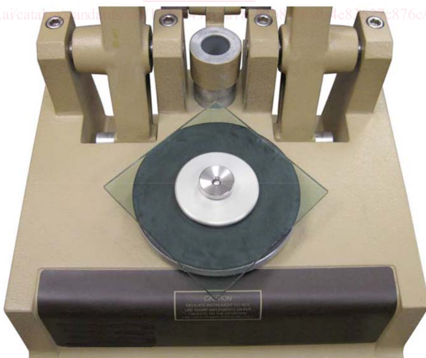
FIG. 3 Specimen Mounting
