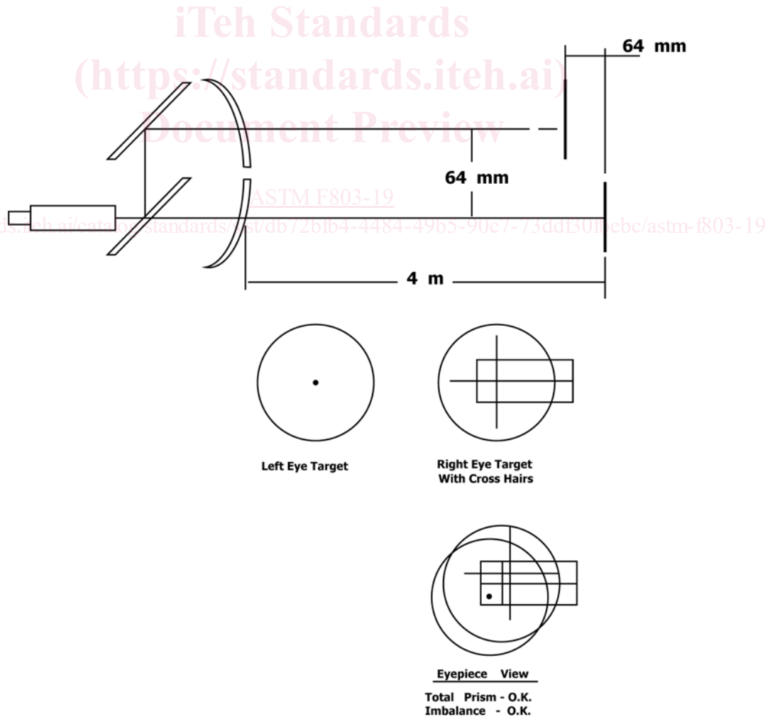
FIG. 1 Alternate Prism Test Set-Up (See 9.8.1)
