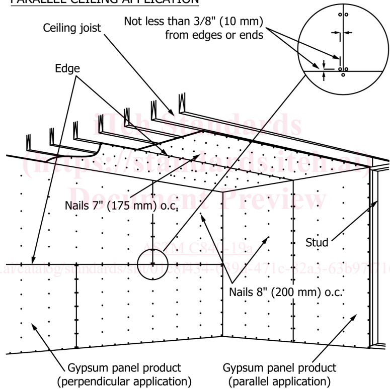
FIG. 2 Single Nailing
