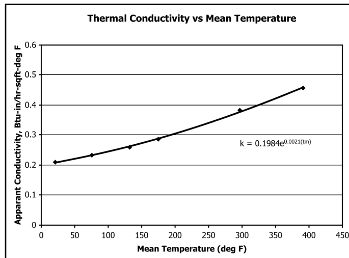
FIG. 2 Thermal Conductivity vs. Mean Temperature
