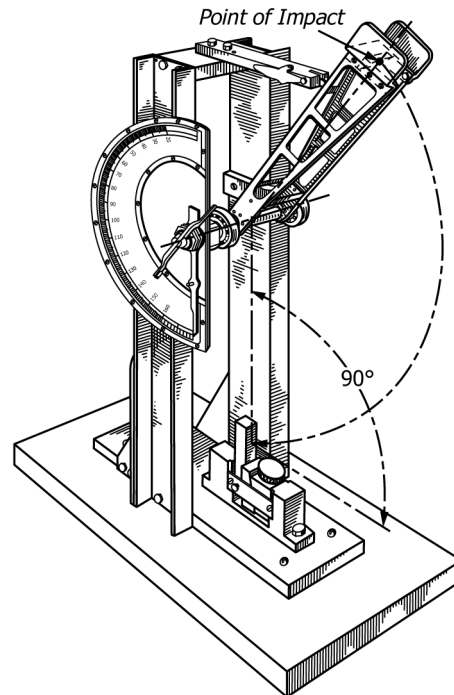
FIG. 1 Cantilever Beam Impact Test Equipment
