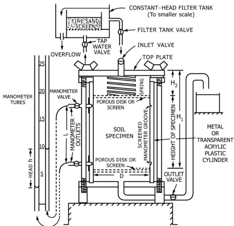
FIG. 1 Constant-Head Permeameter
