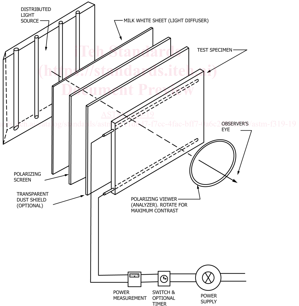
FIG. 1 Typical Arrangement for Polarized Light Method
