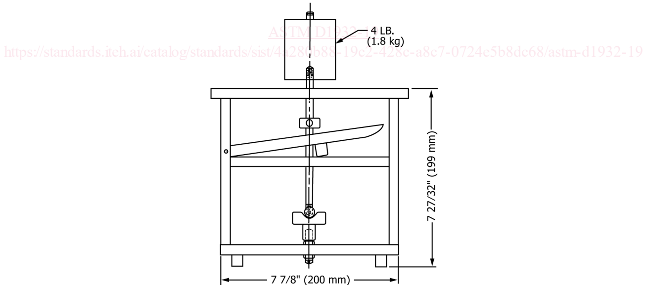
FIG. 2 Curved Electrode and Holder
