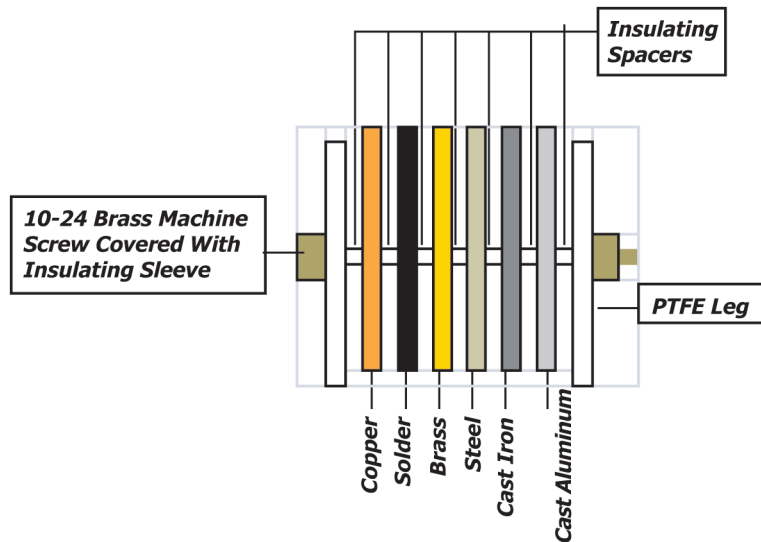
FIG. 2 Test Specimens Arrangement
