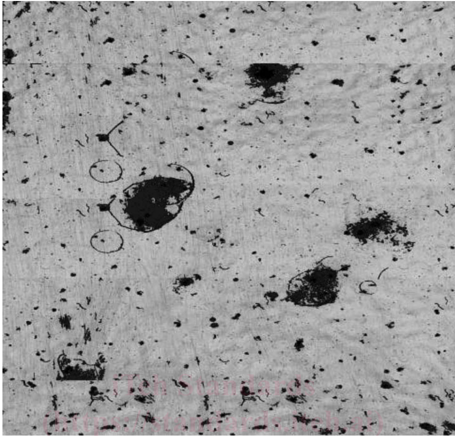
FIG. X1.3 Digitally Enhanced Photograph of Acid Etch Produced by the Exposure Described in This Standard (actual size 4 × 6 in. [10.16 × 15.24 cm]) 10 Rating 4.97 % Defects
