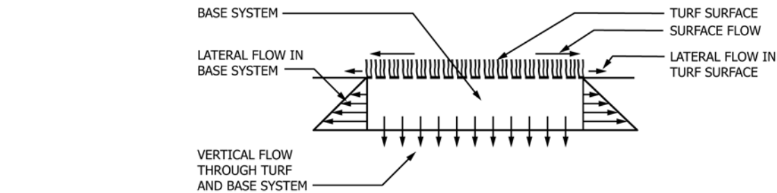
FIG. 1 Basic Flow Regime Diagram
