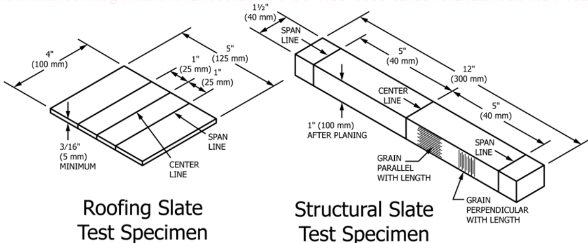
FIG. 1 Specimens and Preferred Type of Loading Application and Support Blocks for Determining the Breaking Load and Modulus of Rupture of Slate
