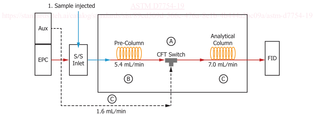
FIG. 3 Fluidic Switch Schematic—Oxygenate Transfer
