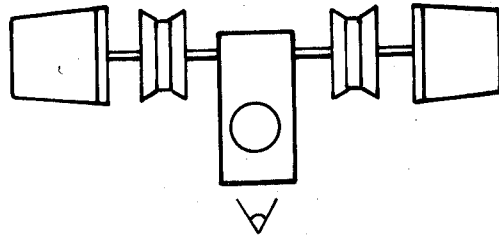
a) Type 1 – Symmetrical double cable-lifter windlass, integral power
