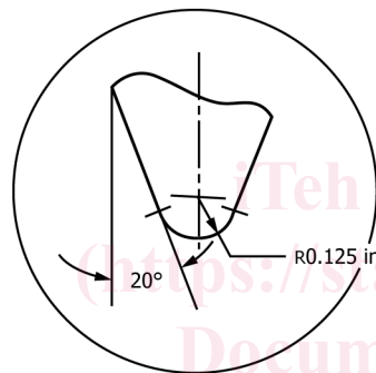
FIG. 3 Impactor Head Configuration H.25 Specimen Support Detail
