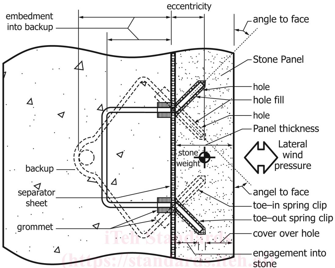
FIG. 6 Spring-Clip Cast-in Anchorage – anchor in horizontal or vertical plane can support gravity and lateral loads (prefer horizontal clip orientation to support combined loads)
