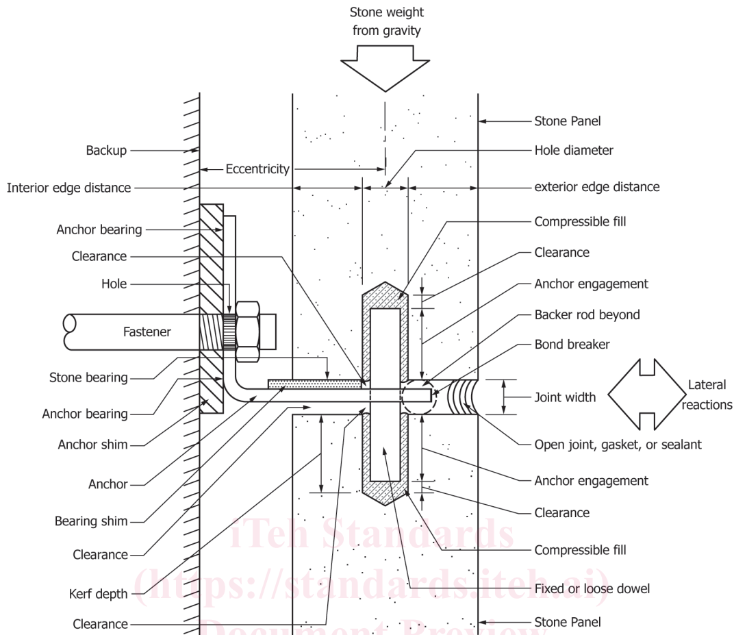
FIG. 78 Dowel Anchorage (brake-formed version) to support combined gravity plus lateral reactions
