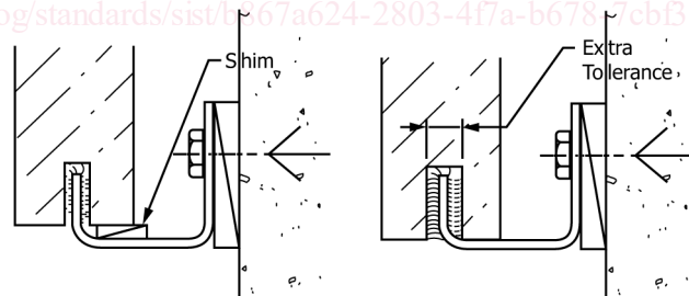
FIG. 3 Point Loading Prevention (continued)
