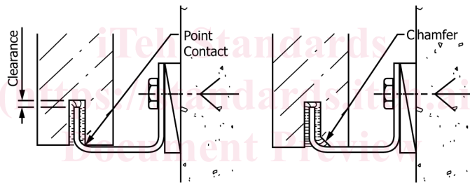
FIG. 3 Point Loading Prevention
