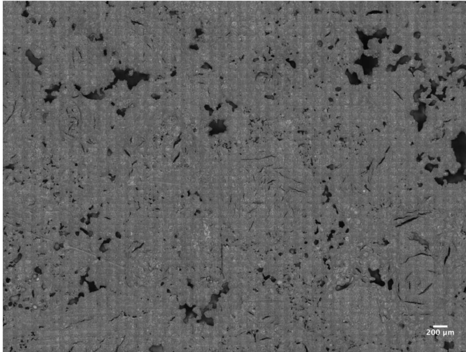
FIG. 1 Micrograph of SGL Group, NBG-18 Graphite
