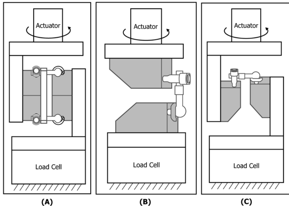
FIG. 4 Diagrams of Possible Test Setups for Rotational Loading of an FP
