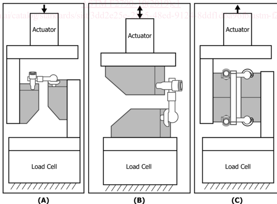
FIG. 3 Diagrams of Possible Test Setups for Translational Loading of an FP
