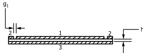
FIG. 3 Glass Specimen with Three-Terminal Electrodes
