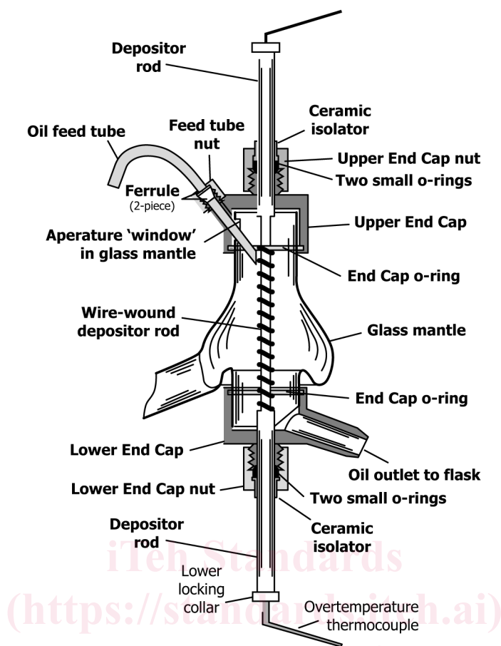
FIG. 5 Insertion of Oil Inlet Tube (Cut-away View)
