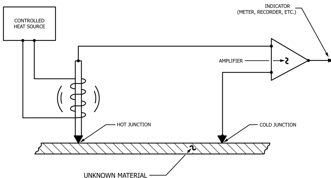
FIG. 1 Typical Circuit Used in Thermoelectric Material Sorting Instruments
