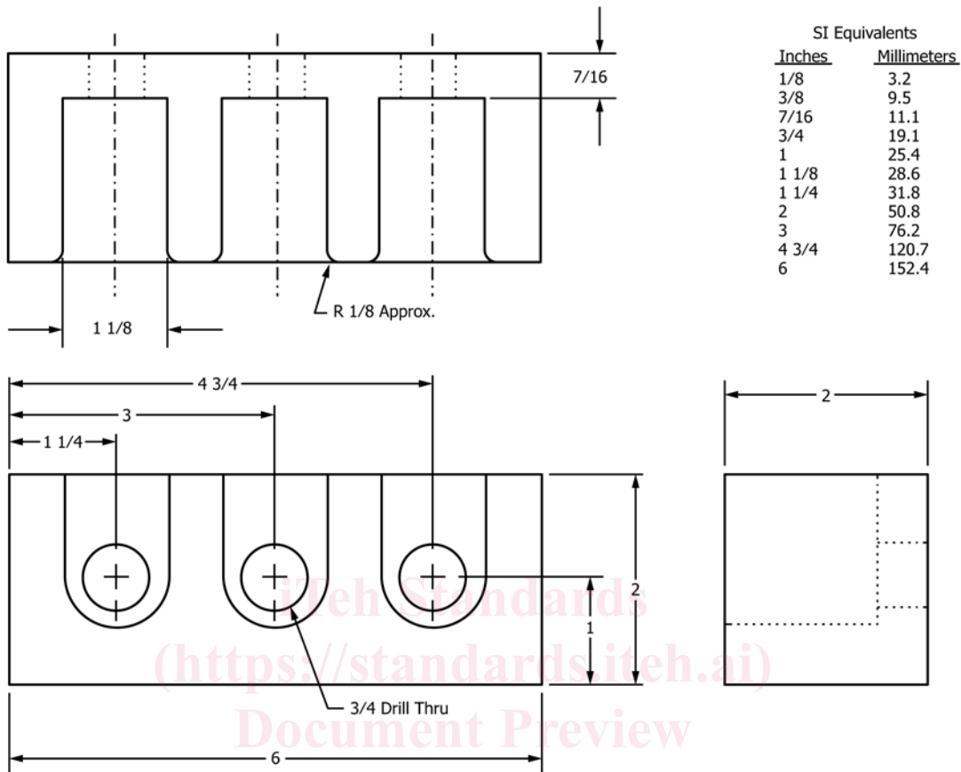
ASTM D6396-99(2020) FIG. 1 3/8 Pipe Tee Assembly Block
