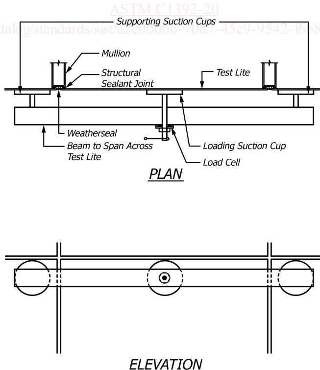
FIG. 1 Schematic of Field Loading Device
