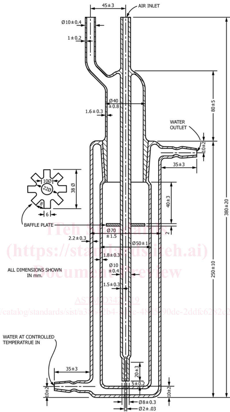
FIG. 2 Test Vessel
