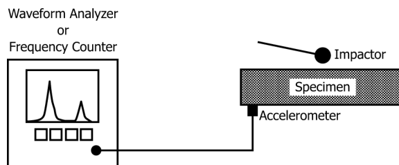
FIG. 2 Schematic of Apparatus for Impact Resonance Test
