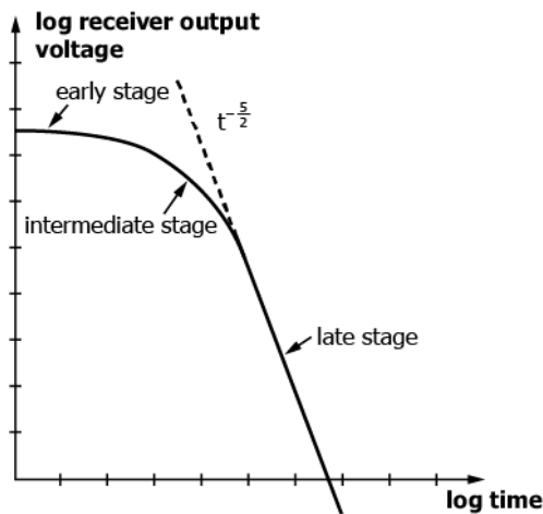
FIG. 4 Typical TEM Receiver Output Voltage Versus Time Plot (5)
