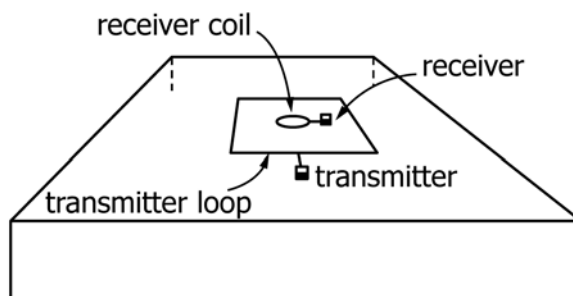
FIG. 1 Typical TDEM/TEM Survey Configuration (5)
