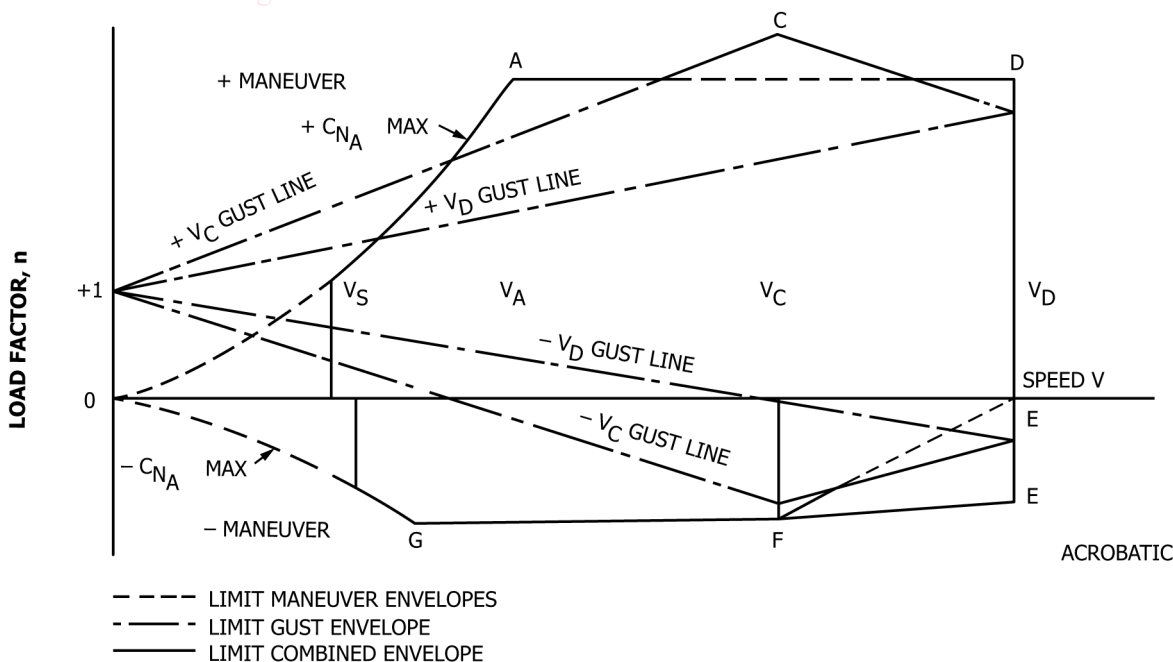
FIG. 1 Flight Envelope
