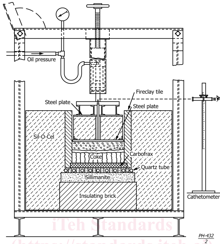
FIG. 1 Sole-Heated Oven
