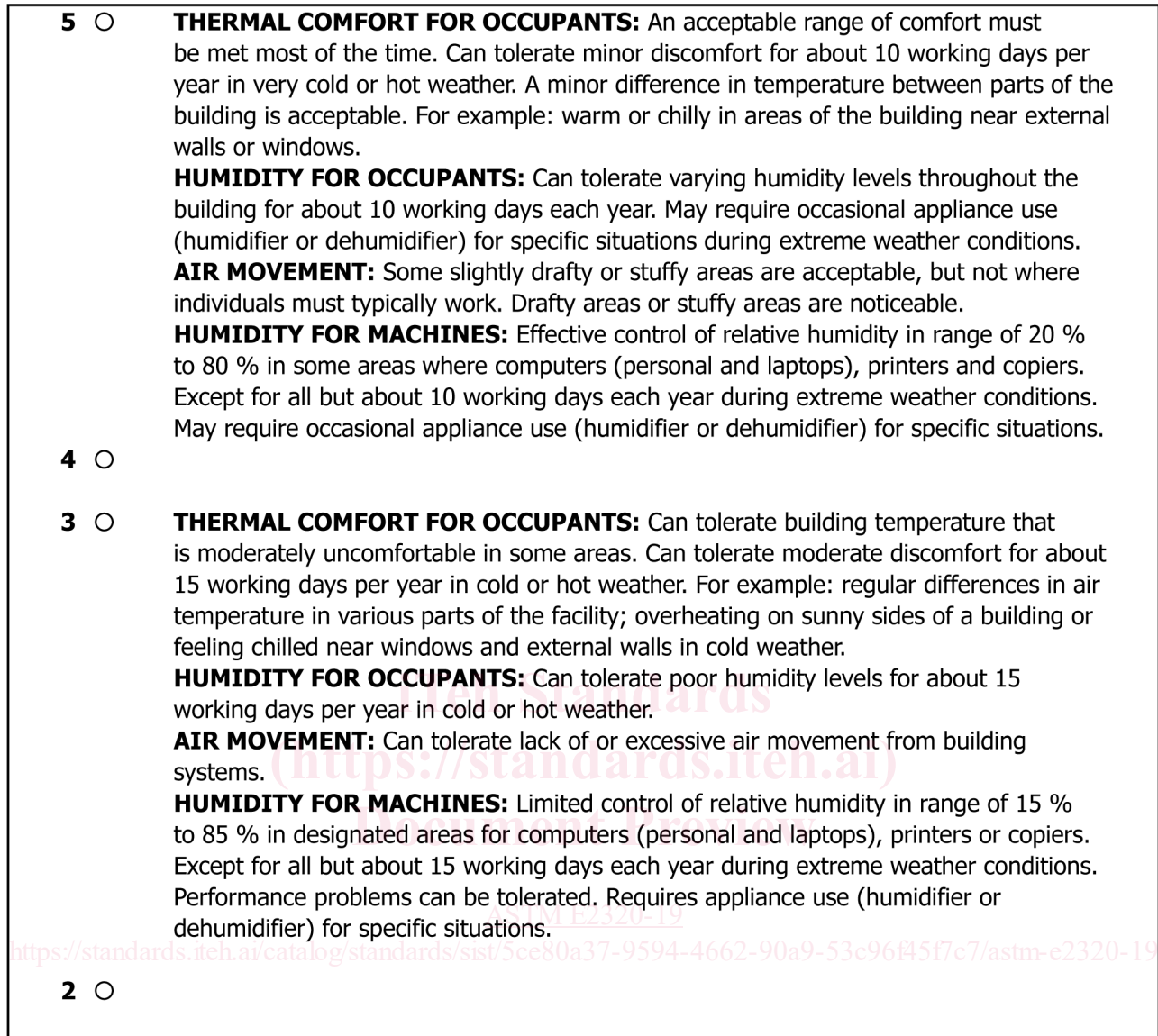
FIG. 21 Demand Scale A.4.2 for Indoor Air Quality Conditions A.4.1 for Information on Temperature and Humidity (continued)
