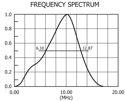
FIG. 1 Test Data Available from Shock Excitation Procedure
