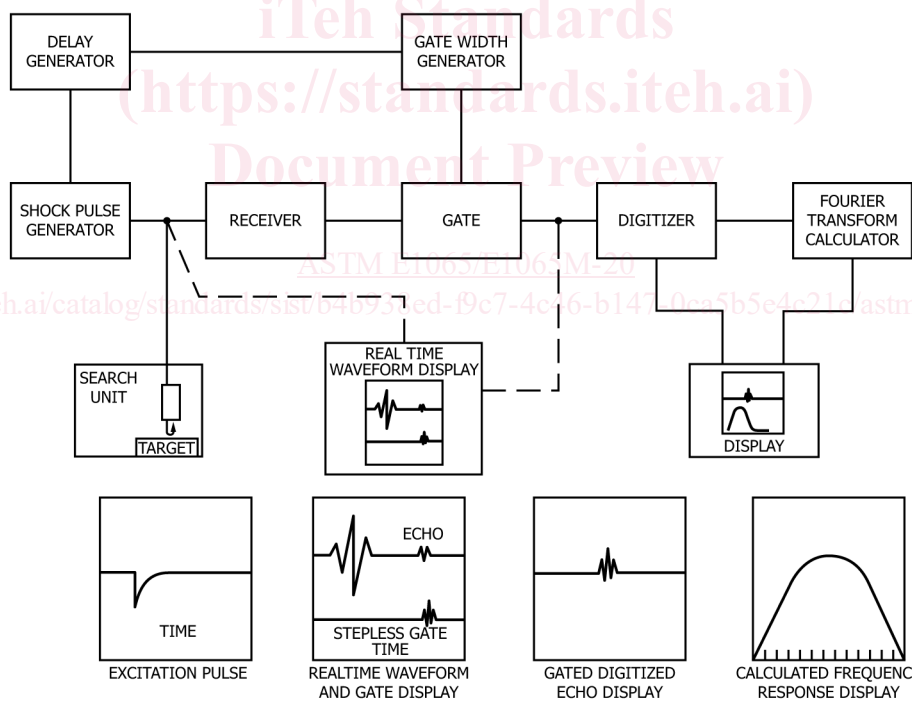
FIG. A1.3 Block Diagram of Shock Excitation System Used to Obtain Digitized rf Waveform Information
