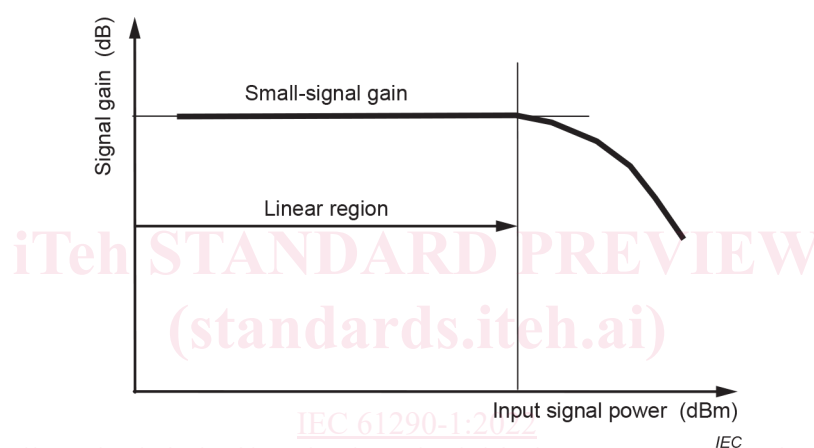
Figure 1 – Typical behaviour of the gain as a function of input signal power
