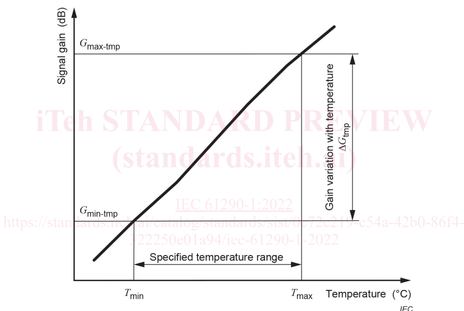
Figure 3 – Typical behaviour of the gain as a function of temperature
