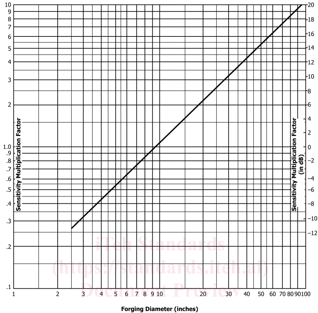
ASTM A418/A418M-15(2020) SENSITIVITY MULTIPLICATION FACTORS FOR SOLID FORGINGS
