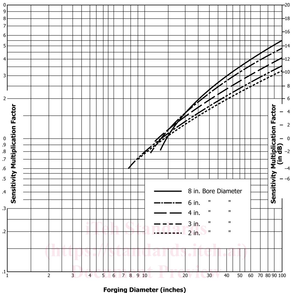
ASTM A418/A418M-15(2020) SENSITIVITY MULTIPLICATION FACTORS FOR BORED FORGINGS
