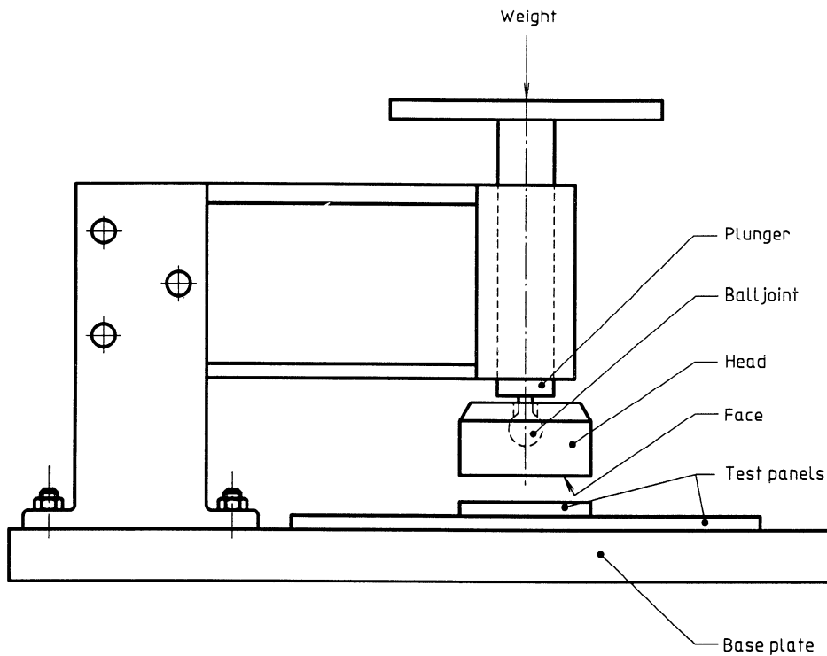
Figure 1 — Example of suitable test apparatus
