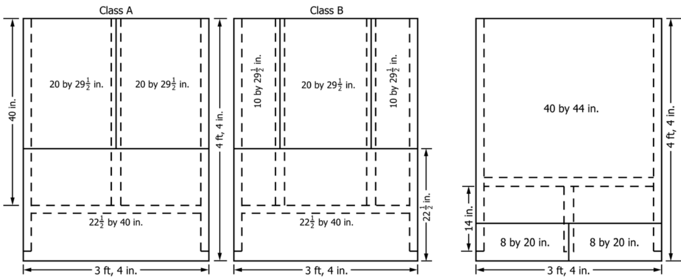
(a) Plywood Decks for Burning Brand Tests
