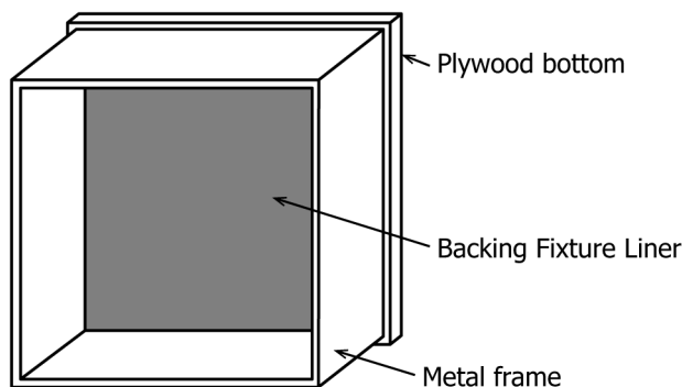
FIG. 21 Backing Fixture
