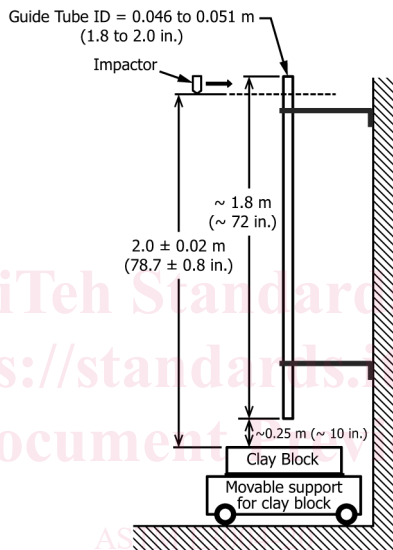
FIG. 54 Example Test Setup
