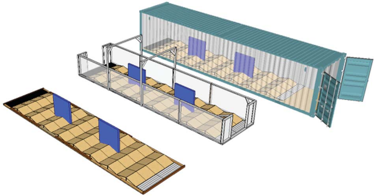
FIG. 8 Various Containment Structures
